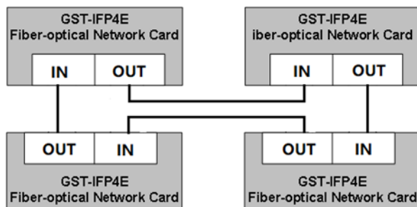
Fig. 1 Fiber Ring Network
